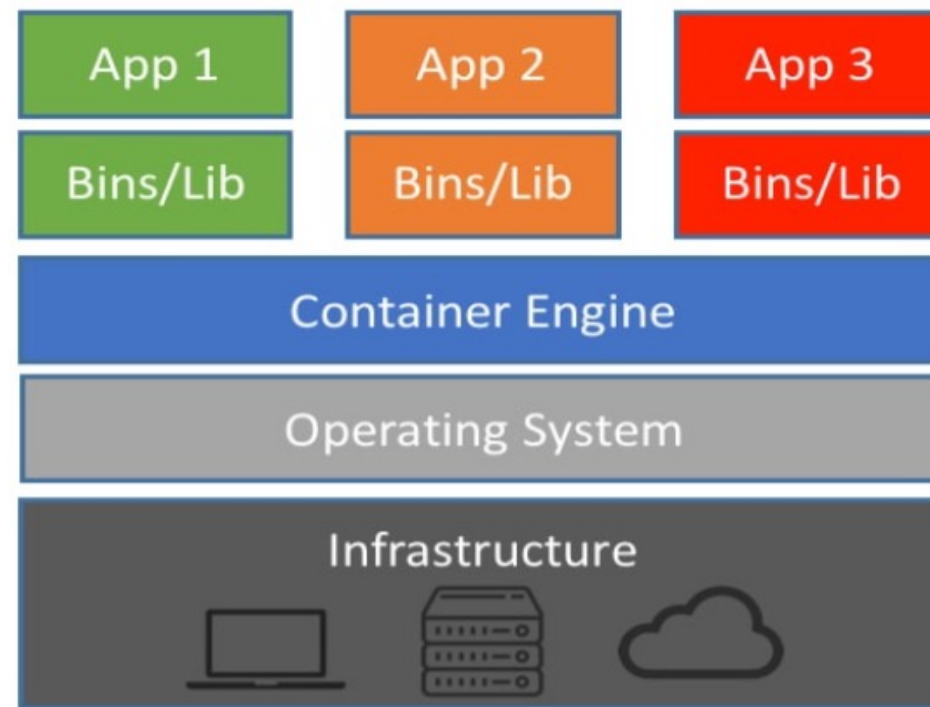
Containers
