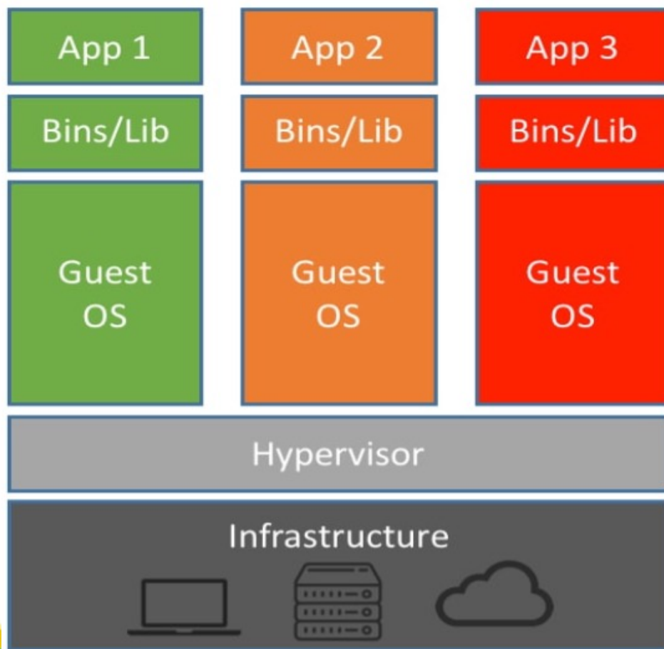
Machine Virtualization
